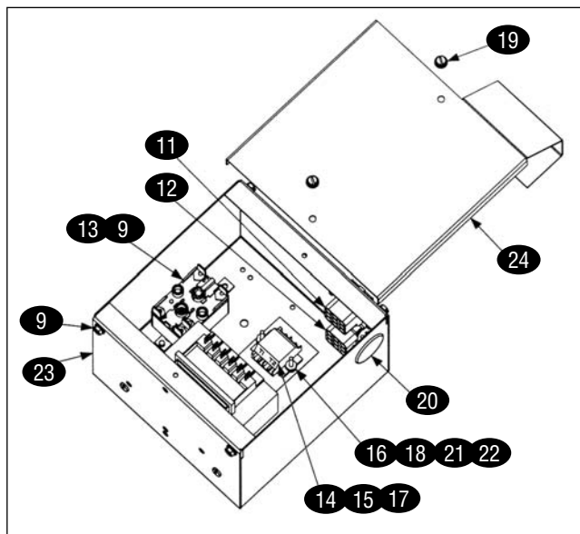
FILTER BOX & ASSEMBLY
